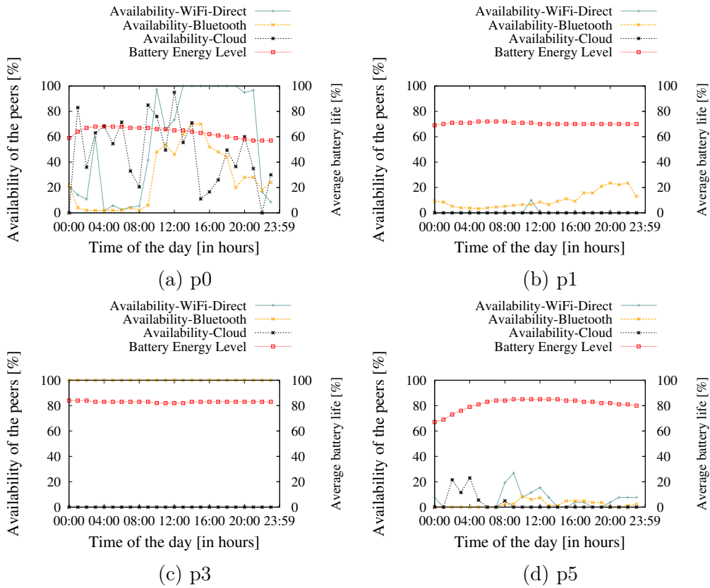
Figure 12: Daily basis availability of offloading support for a) p0, (b) p1, (c) p3, and (d) p5.
