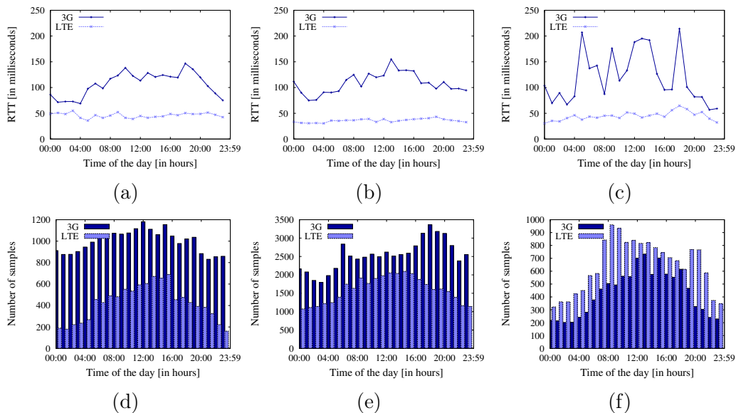
Figure 14: Latency of the network communication by mobile operator for 3G/LTE technologies ((a) DNA, (b) Elisa and (c) Sonera), size of the sample (number of service subscribers (d) DNA, (e) Elisa, and (f) Sonera).
