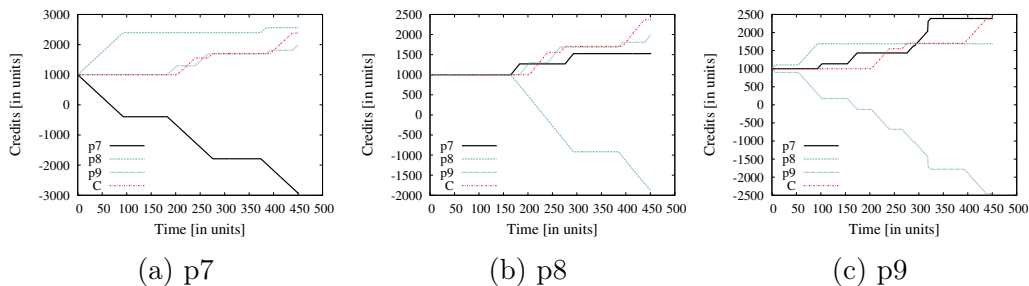
Figure 13: Simulation of credit for (a) p7, (b) p8, and (c) p9.
