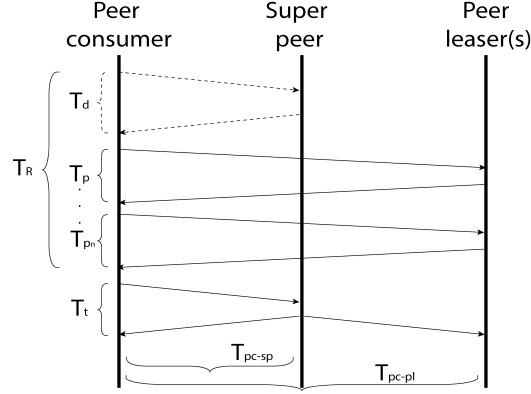
Figure 4: Timestamps and processing procedure of an offloading request in HyMobi.
