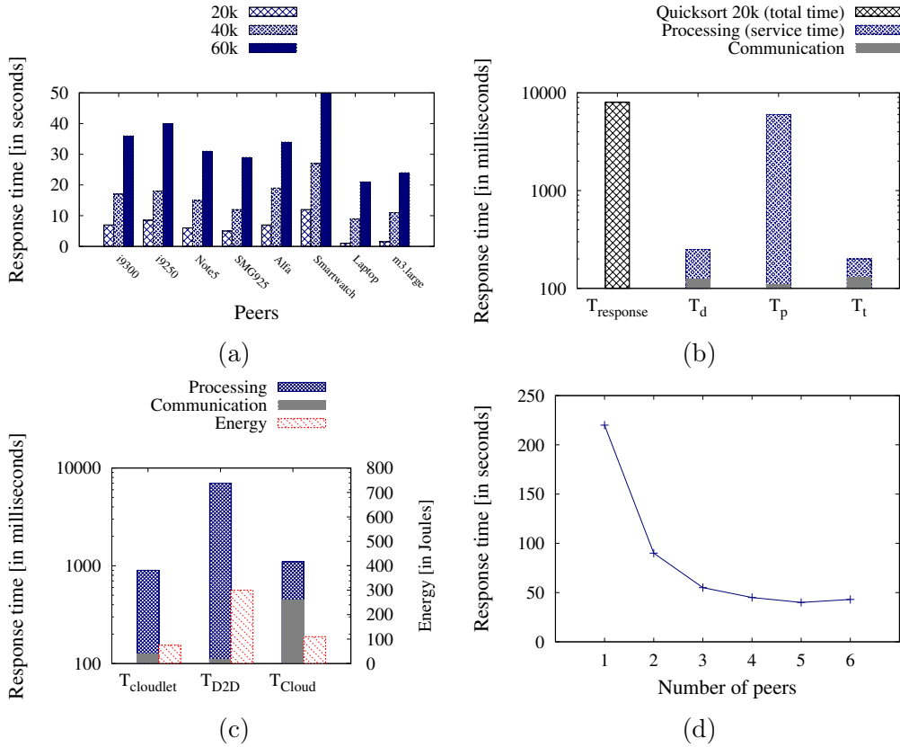
Figure 5: Performance analysis of the offloading process. (a) execution of QuickSort in different devices using different inputs, (b) times of an offloading request throughout the components of the system, (c) execution of a task in different types of peers, and (d) task execution divided into multiple peers.
